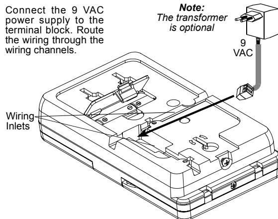
Figure 5: Wiring
